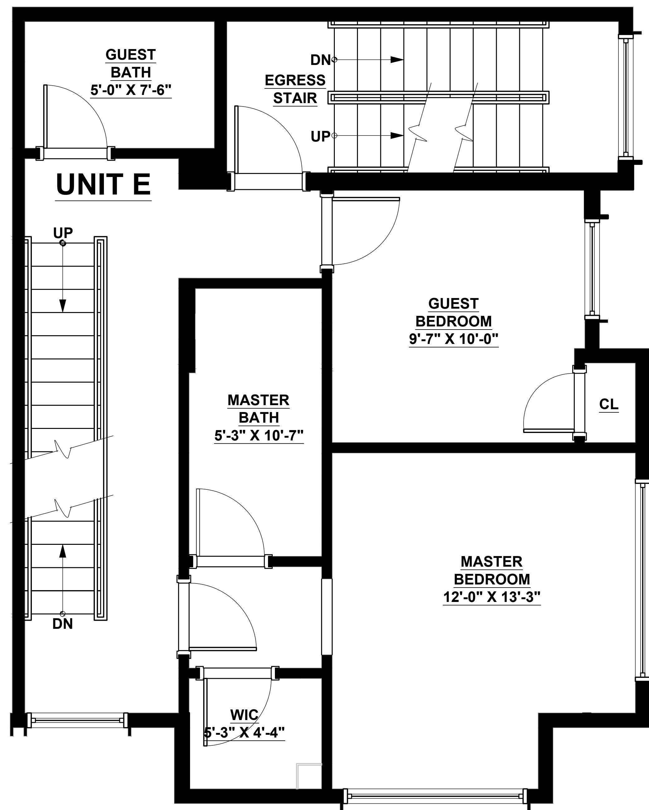
PROPOSED UNIT E PLAN 3/8"=1'-0"
