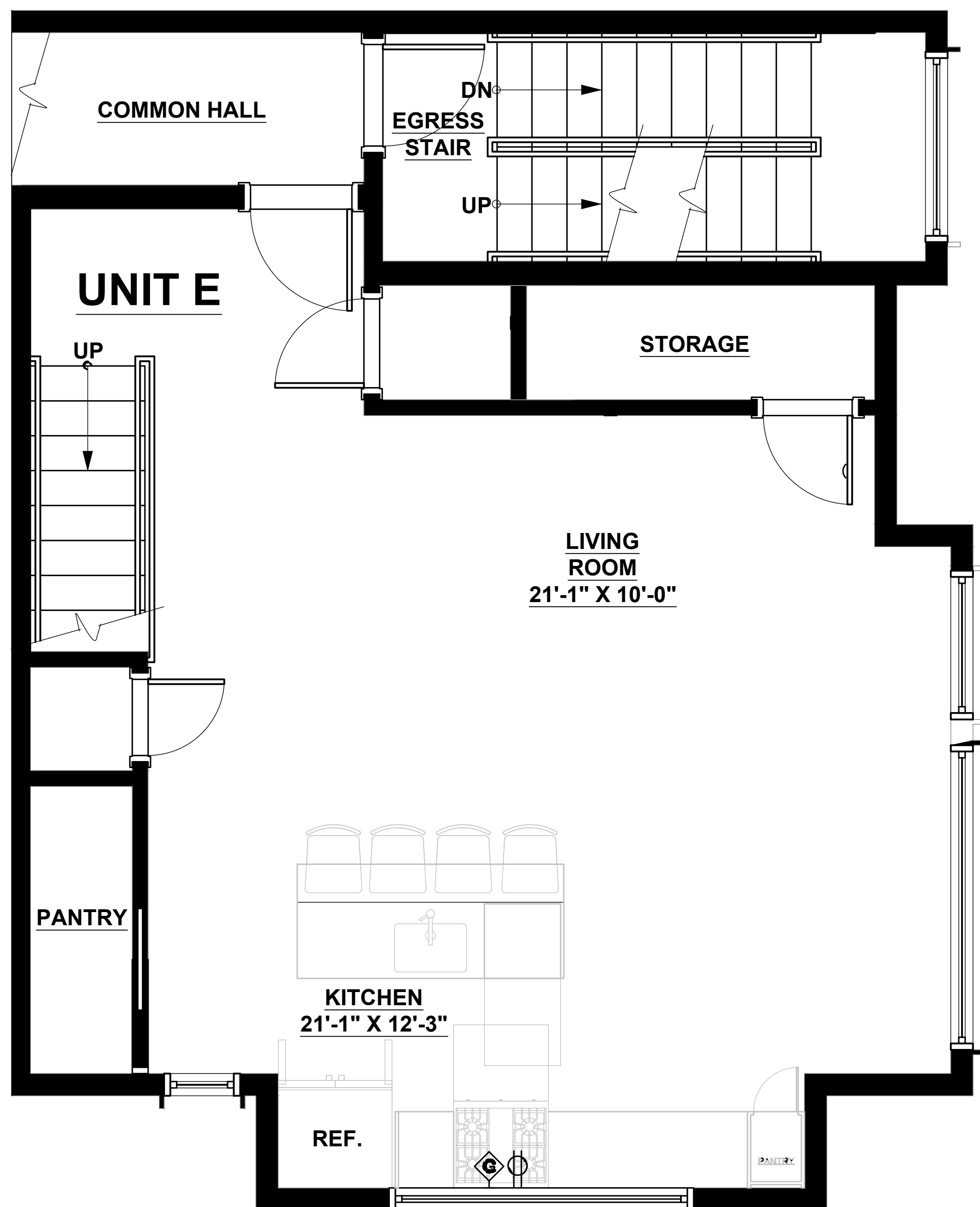
PROPOSED UNIT E PLAN 3/8"=1'-0"
